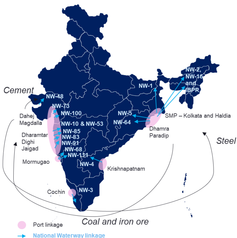
Figure 49: Strategic integration of National Waterways with coastal ports enables multimodal movement of coal, iron ore, cement, and steel across India
